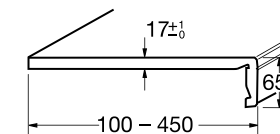
Systemblenden
